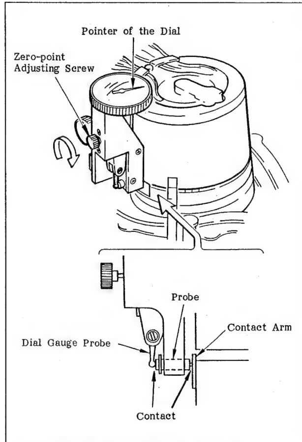
Fig. 5-24 Head Projection Check (4)
